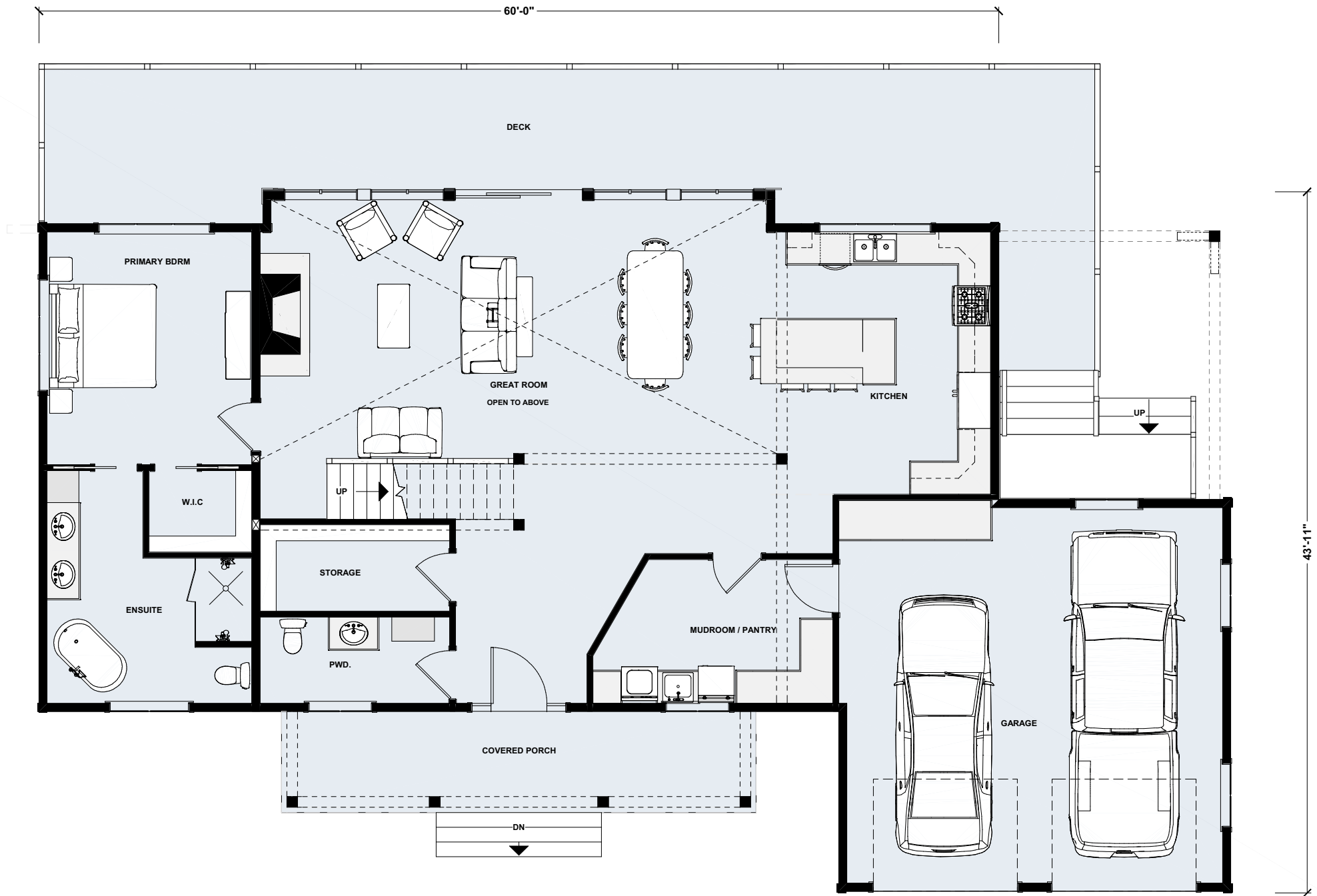
Main Floor Plan | 1,760 sq ft
