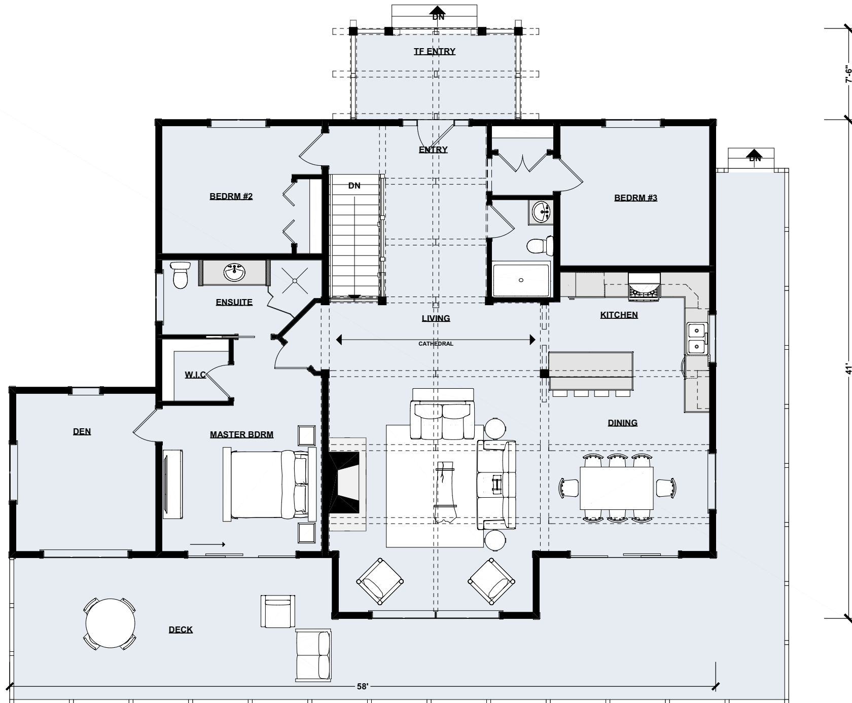
Main Floor Plan | 1,865 sq ft
