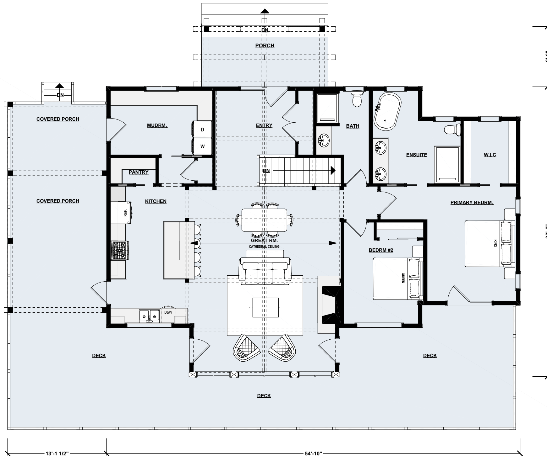
Main Floor Plan | 1,755 sq ft
