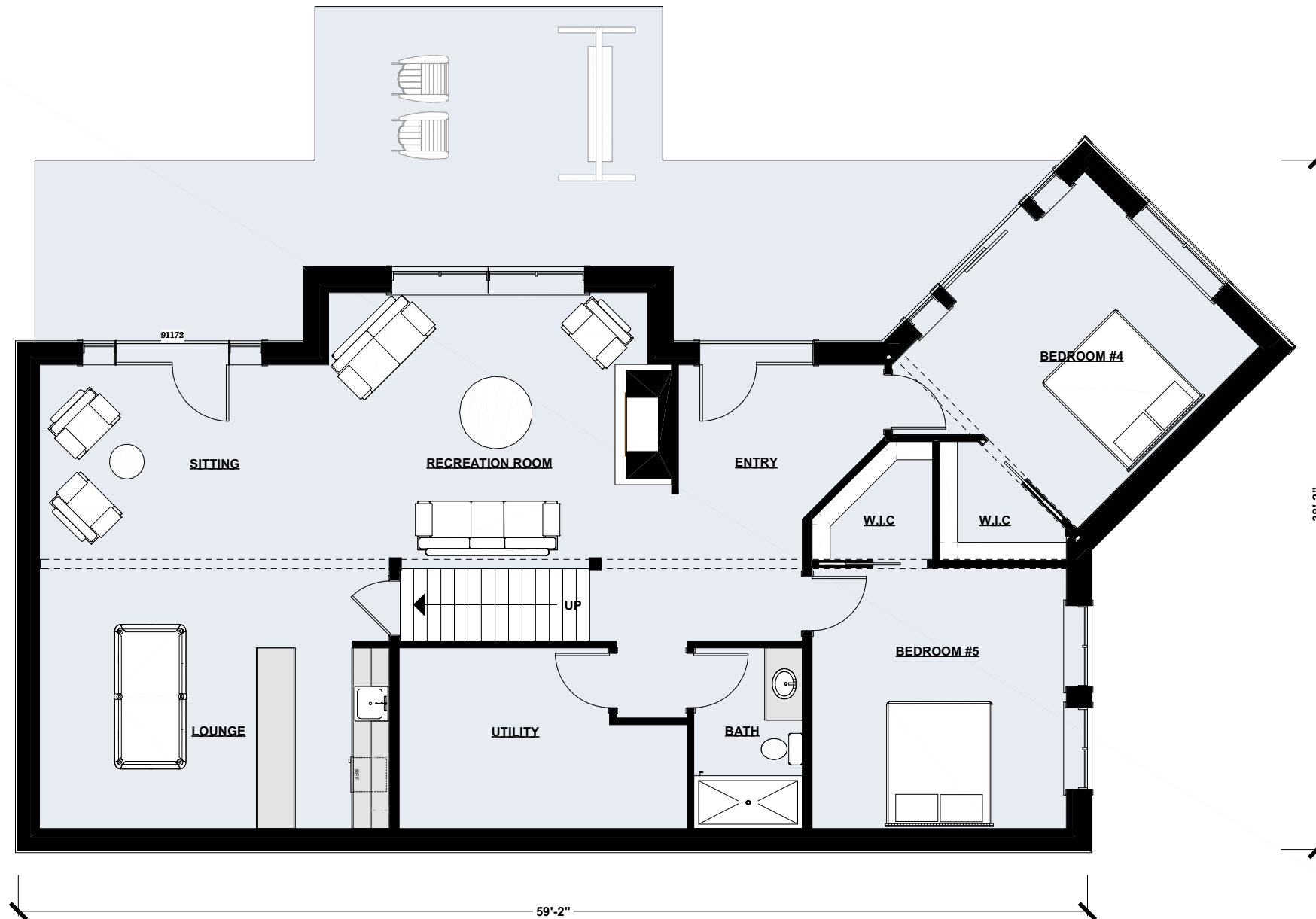
Lower Floor Plan | 1,925 sq ft
