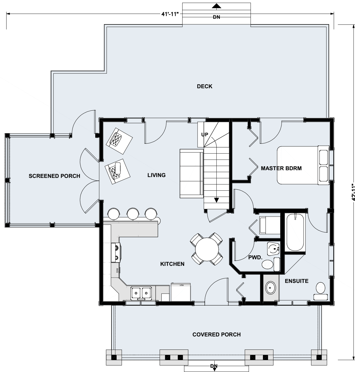
Main Floor Plan | 720 sq ft
