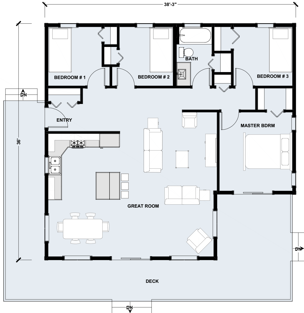
Main Floor Plan | 1260 sq ft
