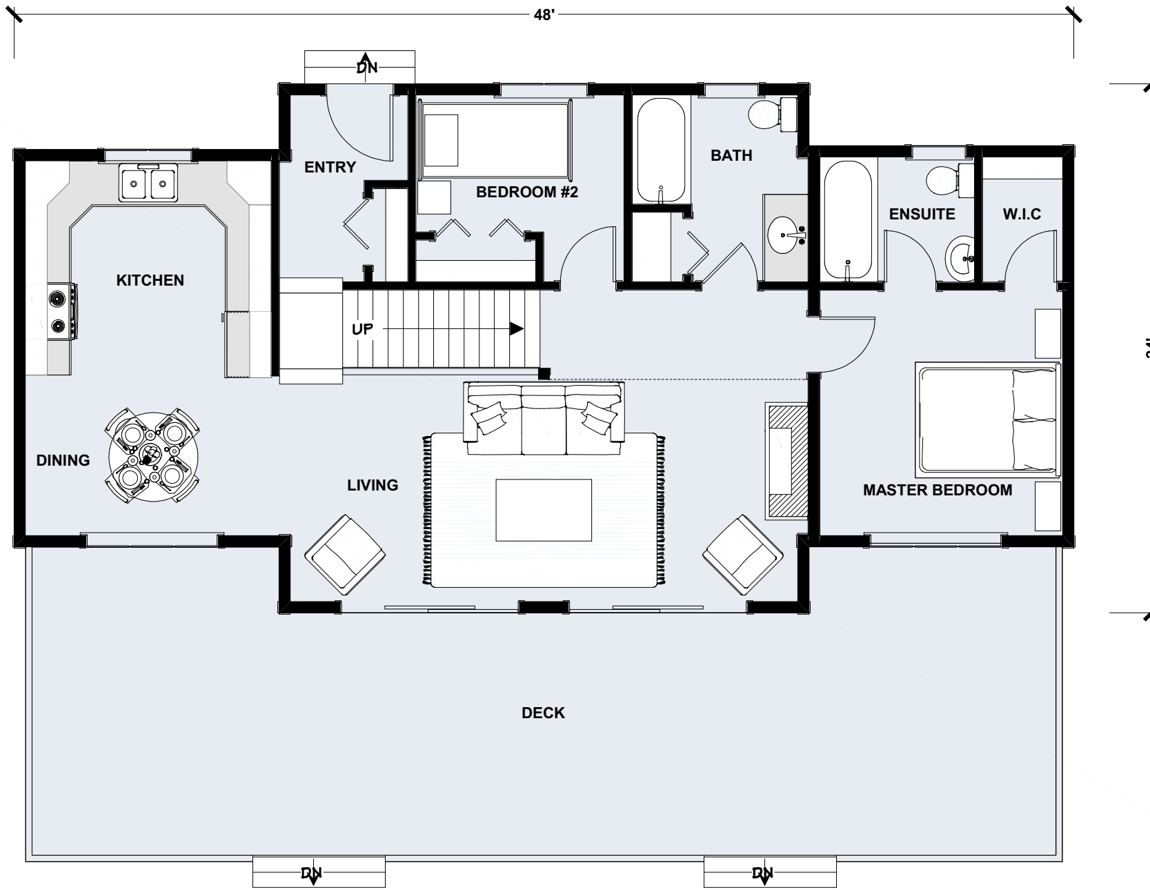
Main Floor Plan | 980 sq ft
