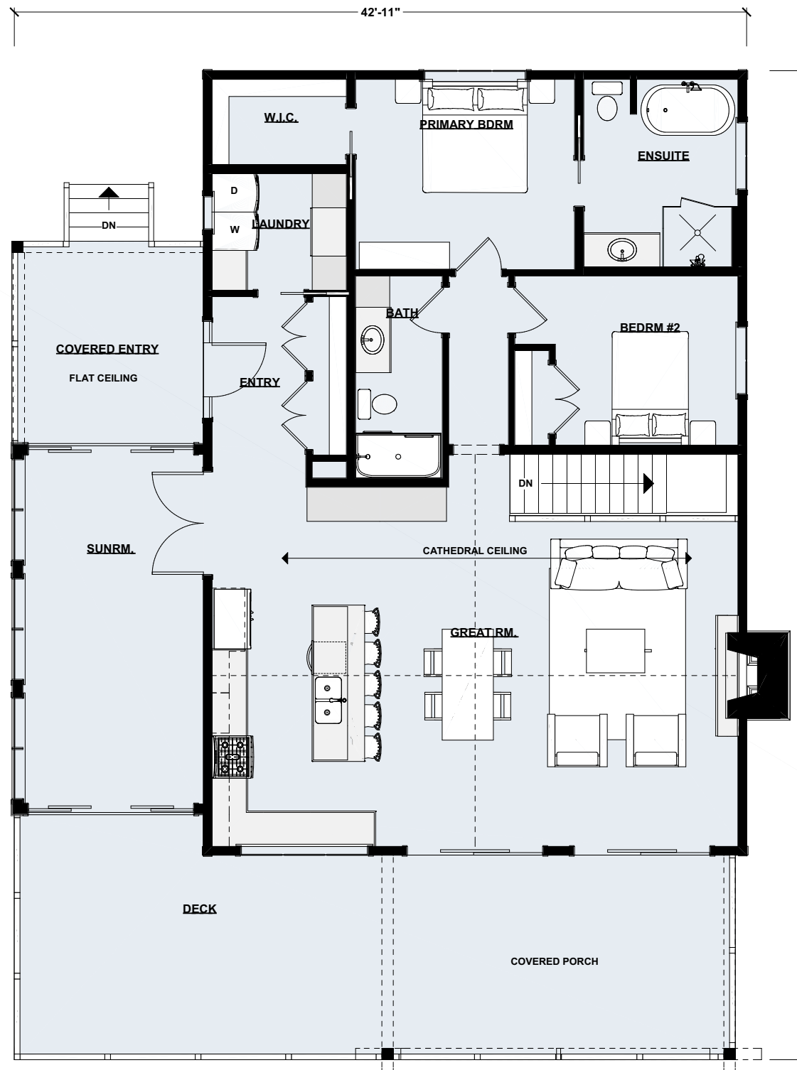
Main Floor Plan | 1,652 sq ft
