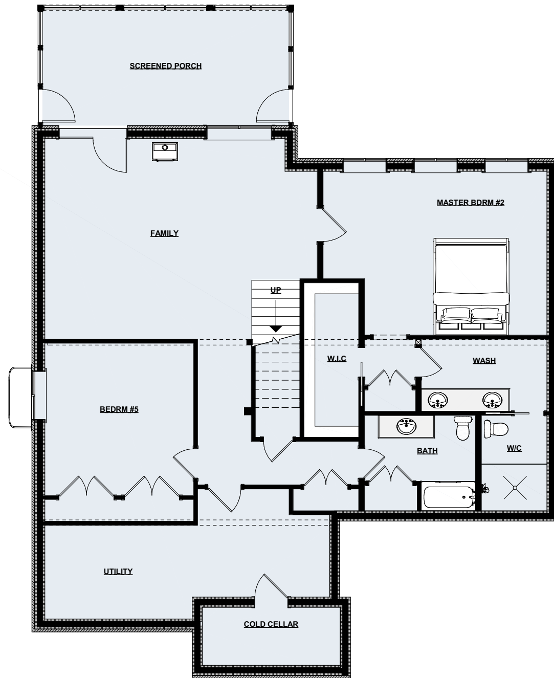
Lower Floor Plan | 1982 sq ft
