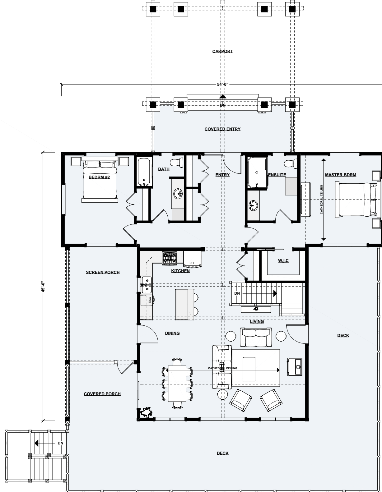
Main Floor Plan | 1,639 sq ft
