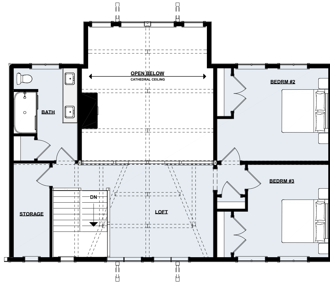
Upper Floor Plan | 947 sq ft
