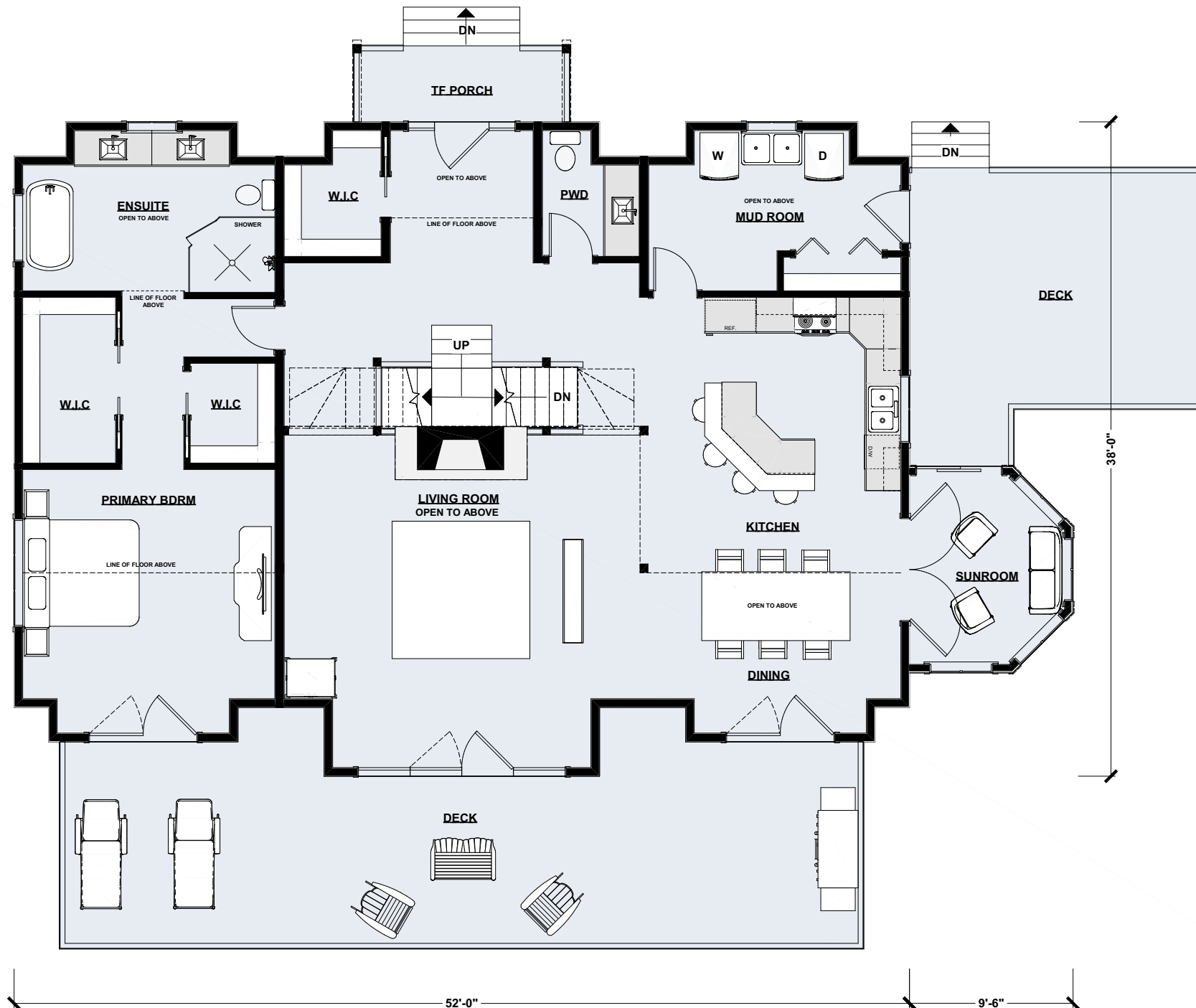
Main Floor Plan | 1,906 sq ft
