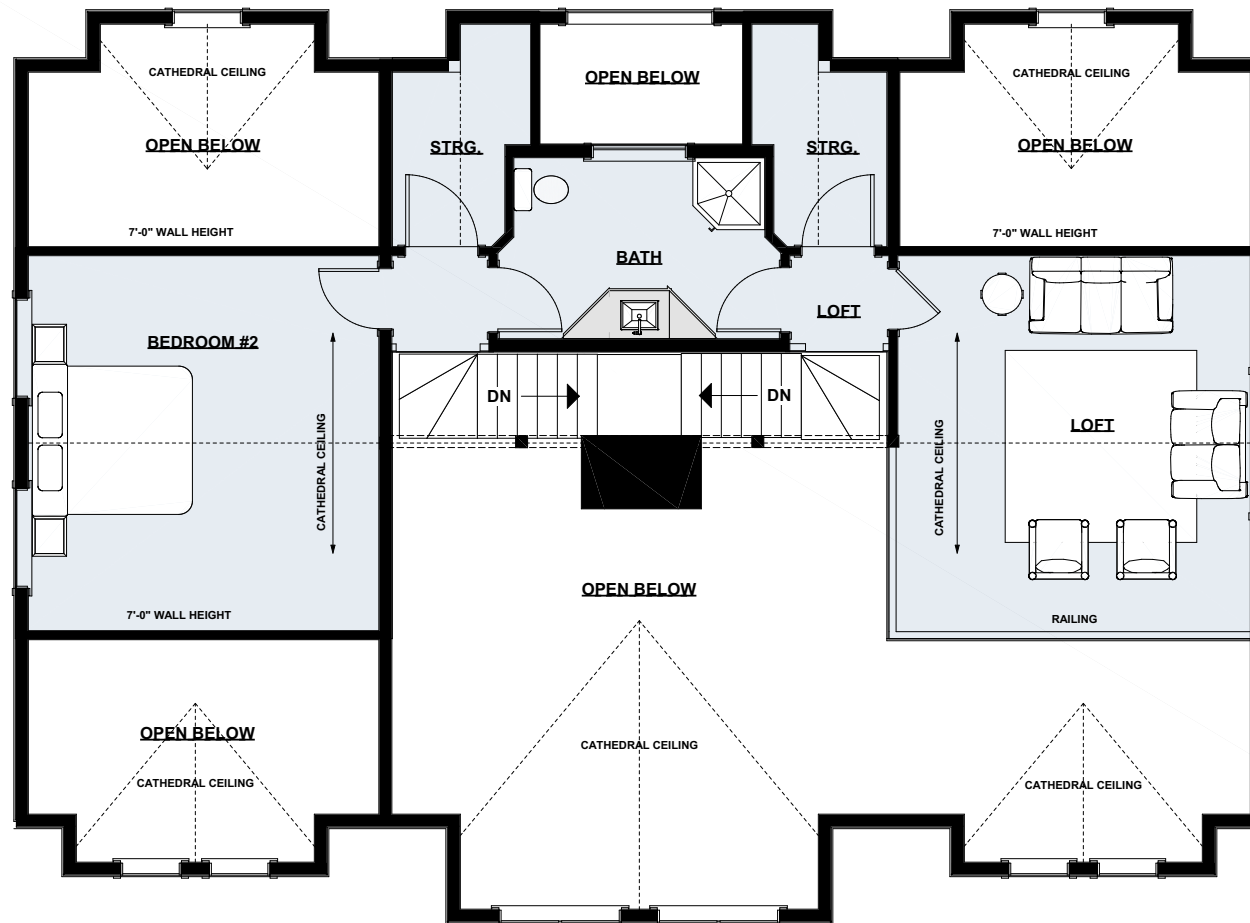
Upper Floor Plan | 753 sq ft
