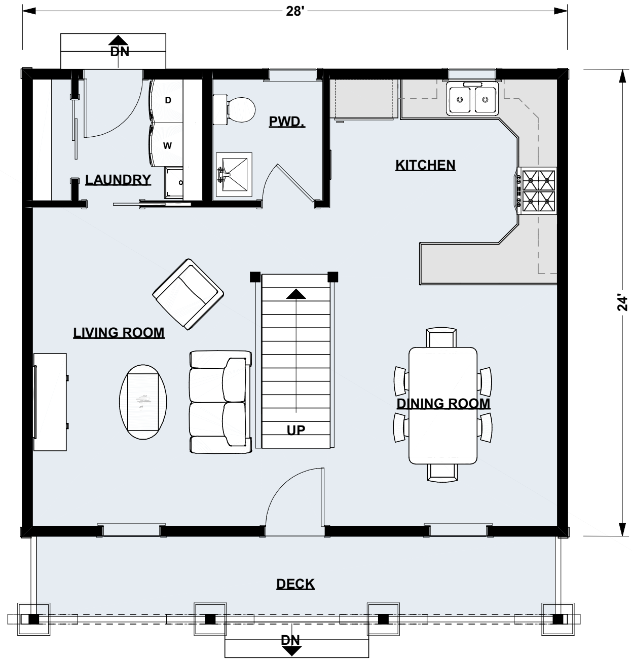
Main Floor Plan | 648 sq ft
