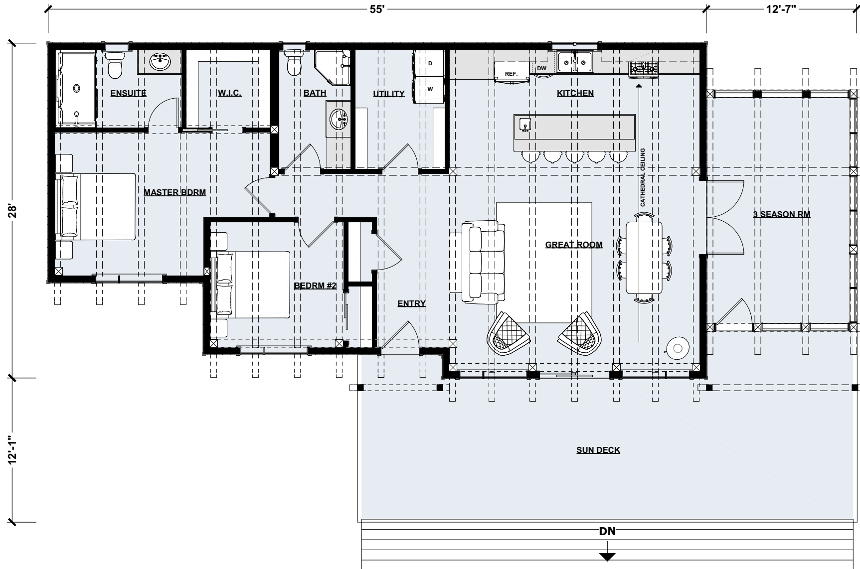
Main Floor Plan | 1,396 sq ft
