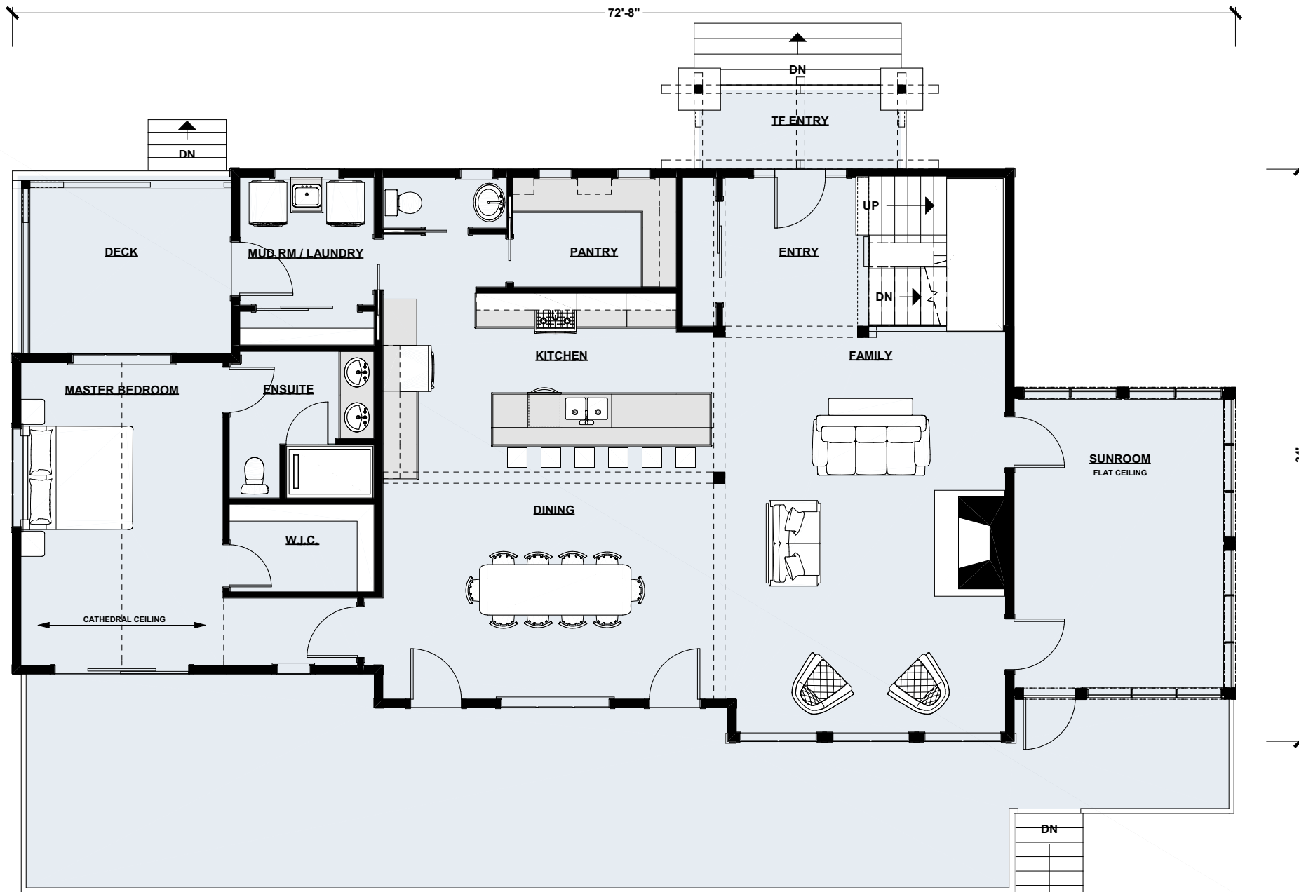
Main Floor Plan | 1,906 sq ft
