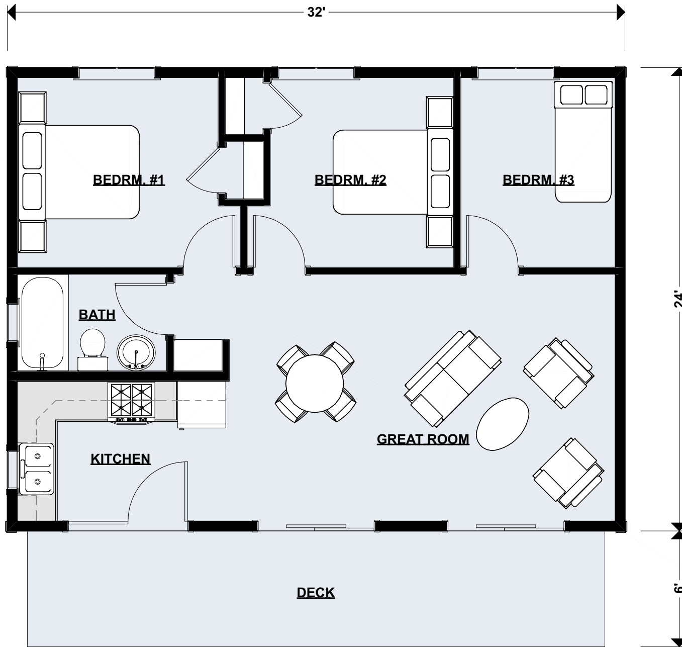
Main Floor Plan | 768 sq ft
