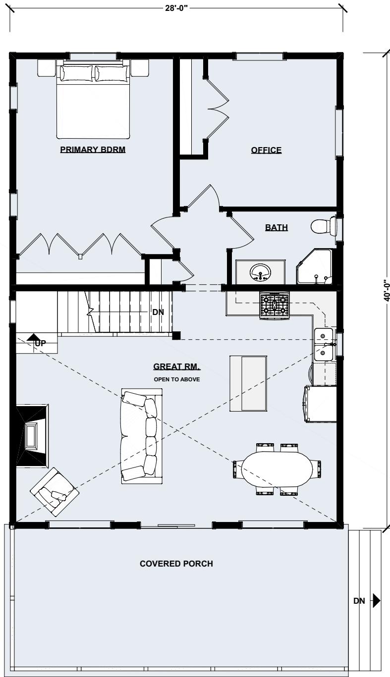
Main Floor Plan | 1,072 sq ft
