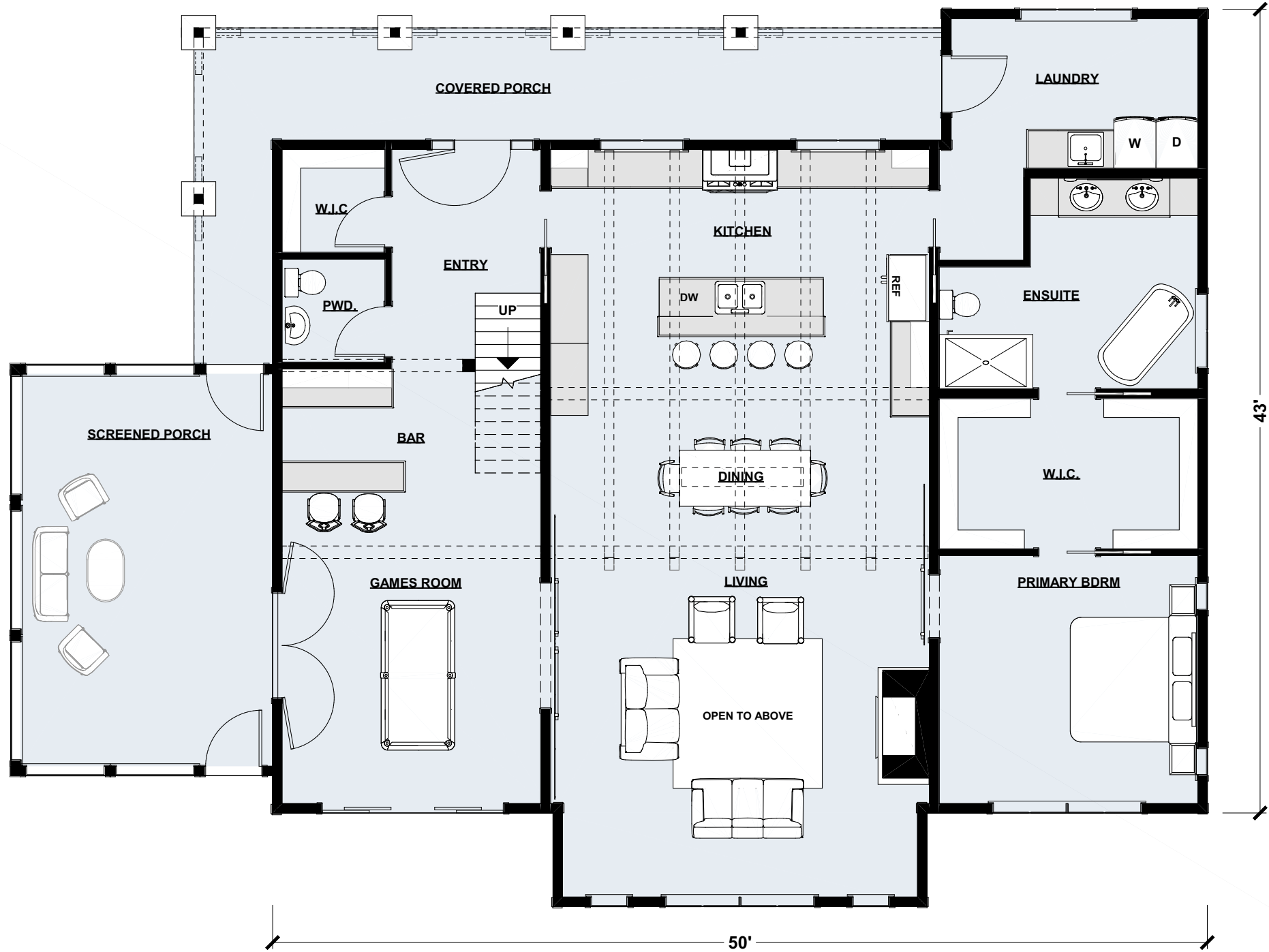
Main Floor Plan | 2,000 sq ft
