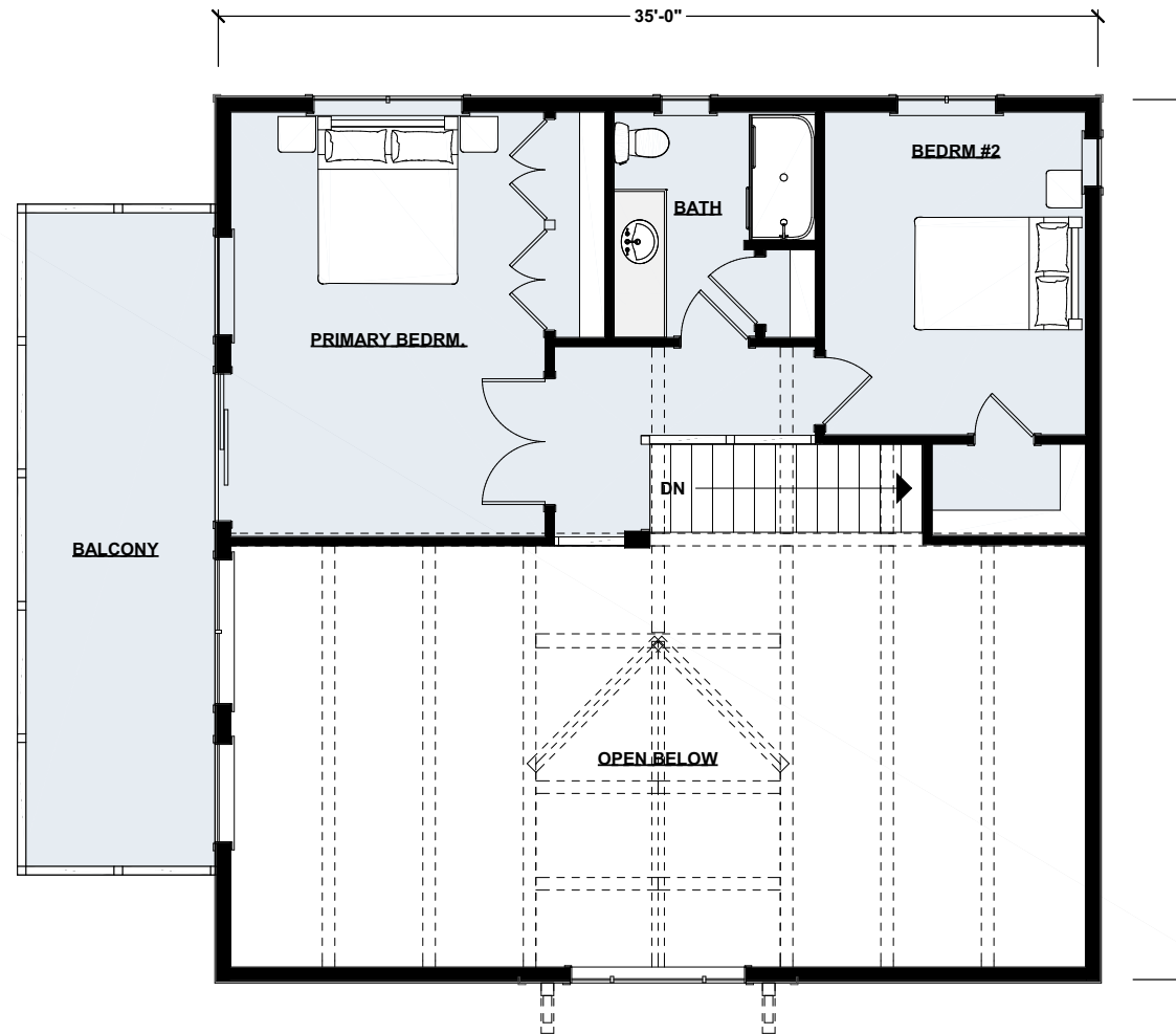
Upper Floor Plan | 576 sq ft
