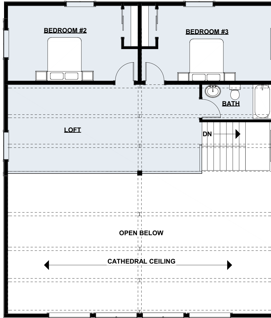
Upper Floor Plan | 889 sq ft
