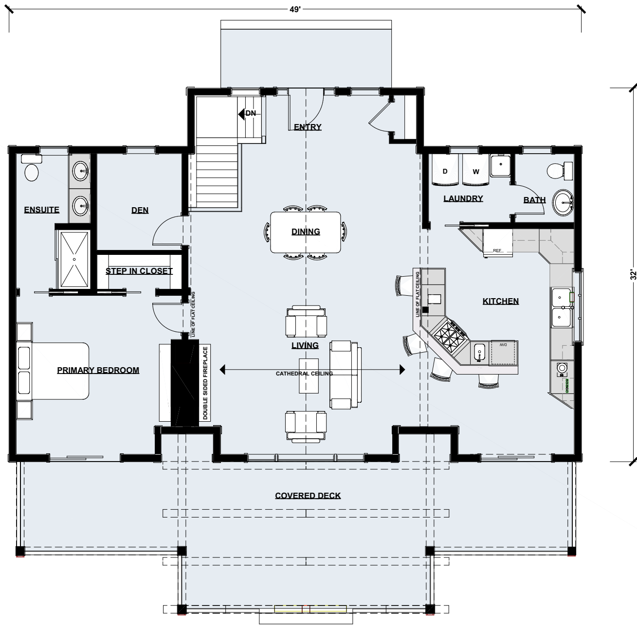
Main Floor Plan | 1,349 sq ft
