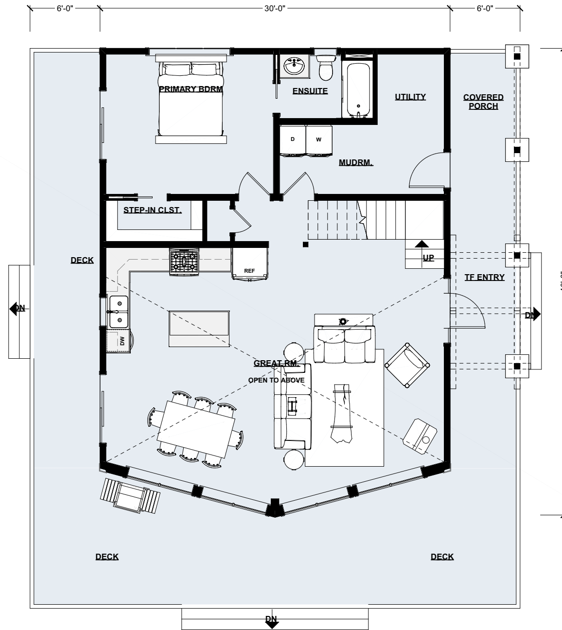
Main Floor Plan | 1,140 sq ft
