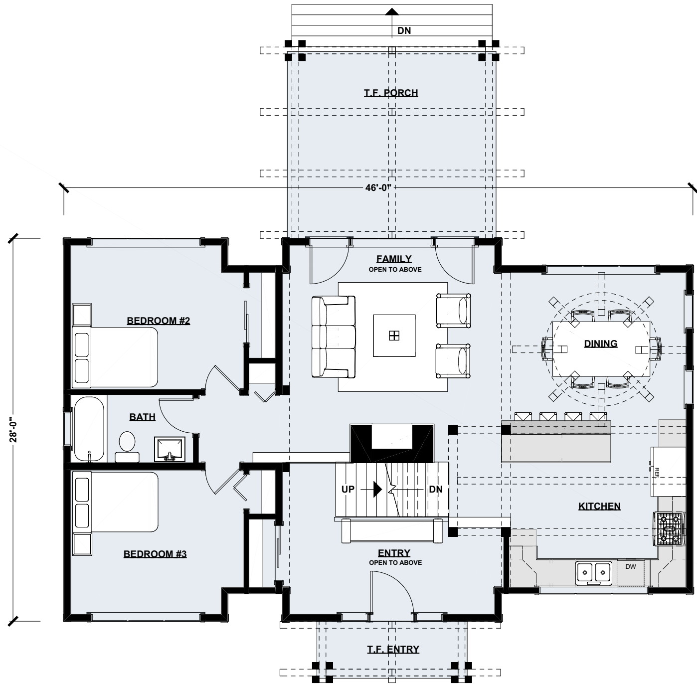
Main Floor Plan | 1,184 sq ft
