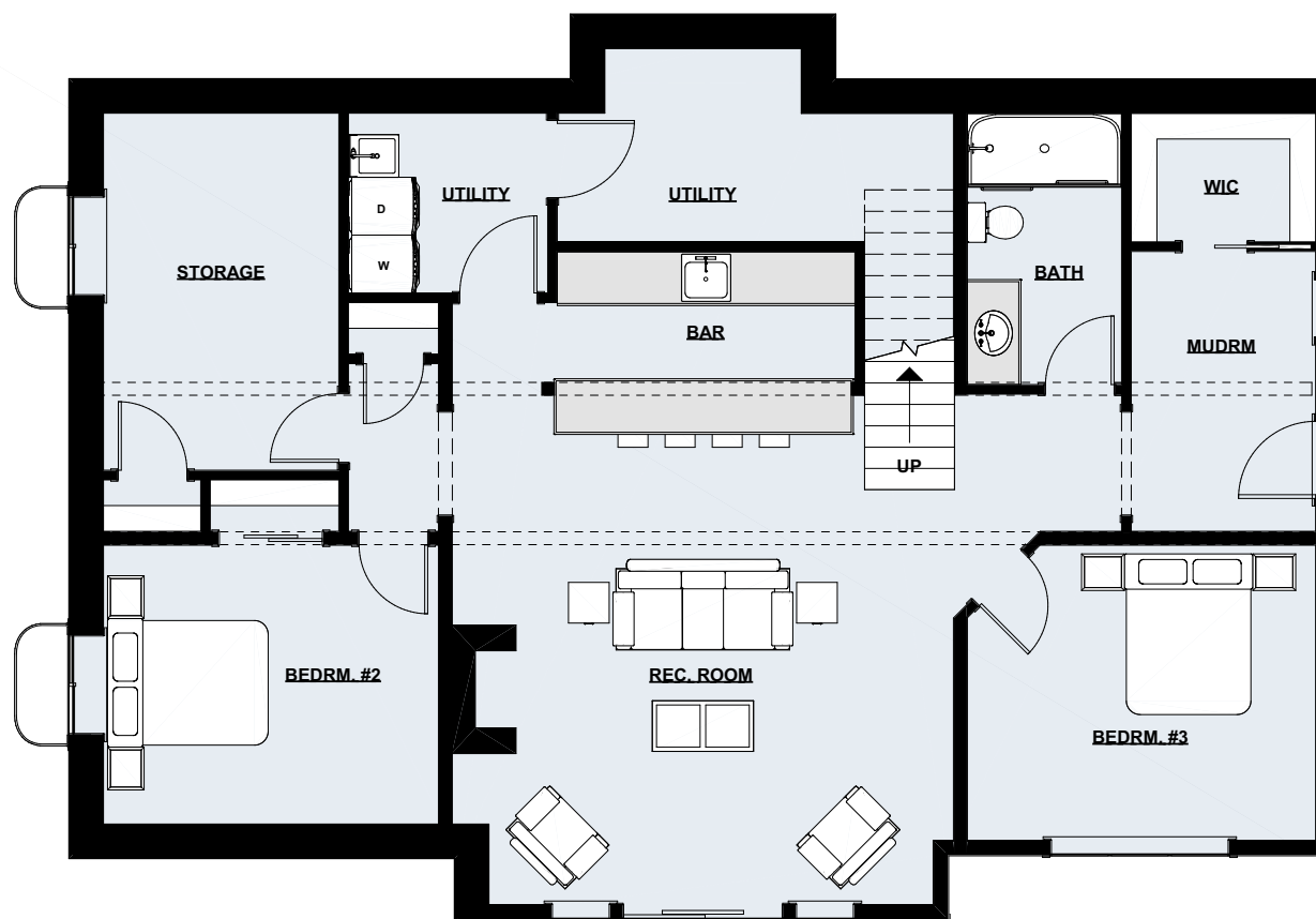
Lower Floor Plan | 1,539 sq ft
