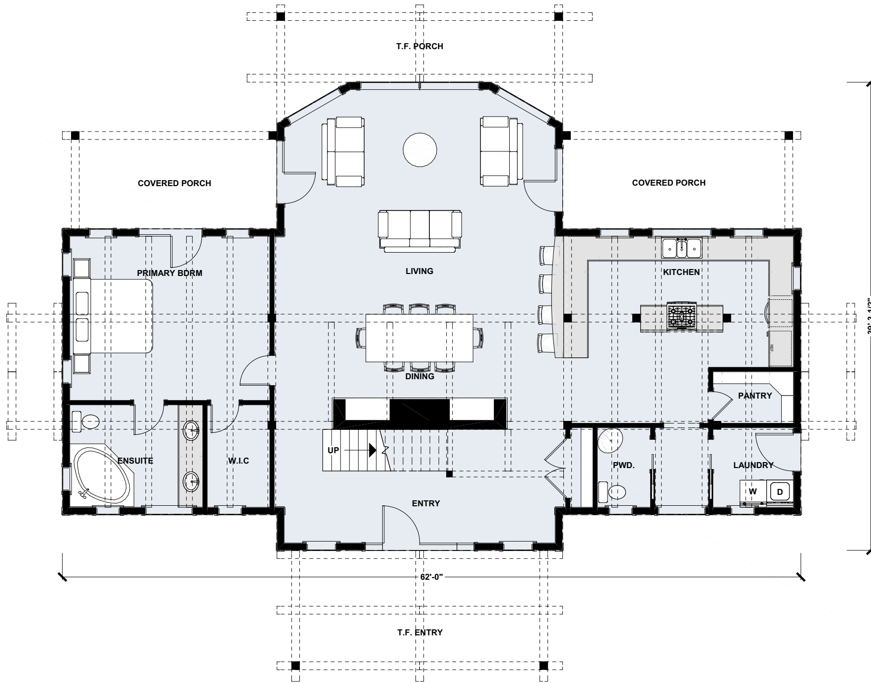
Main Floor Plan | 1,835 sq ft
