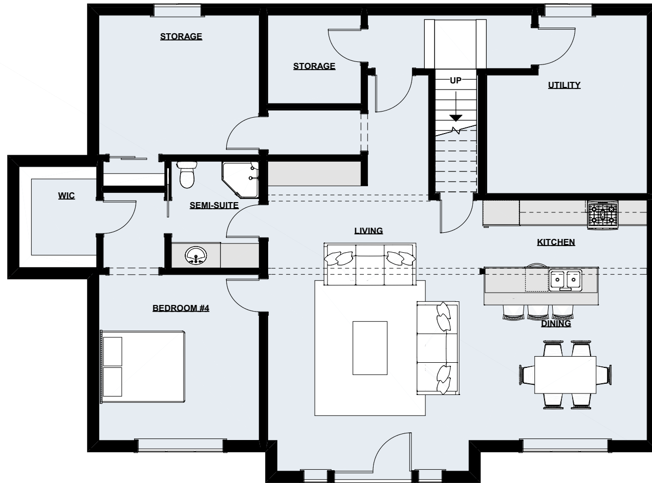
Lower Floor Plan | 1,724 sq ft
