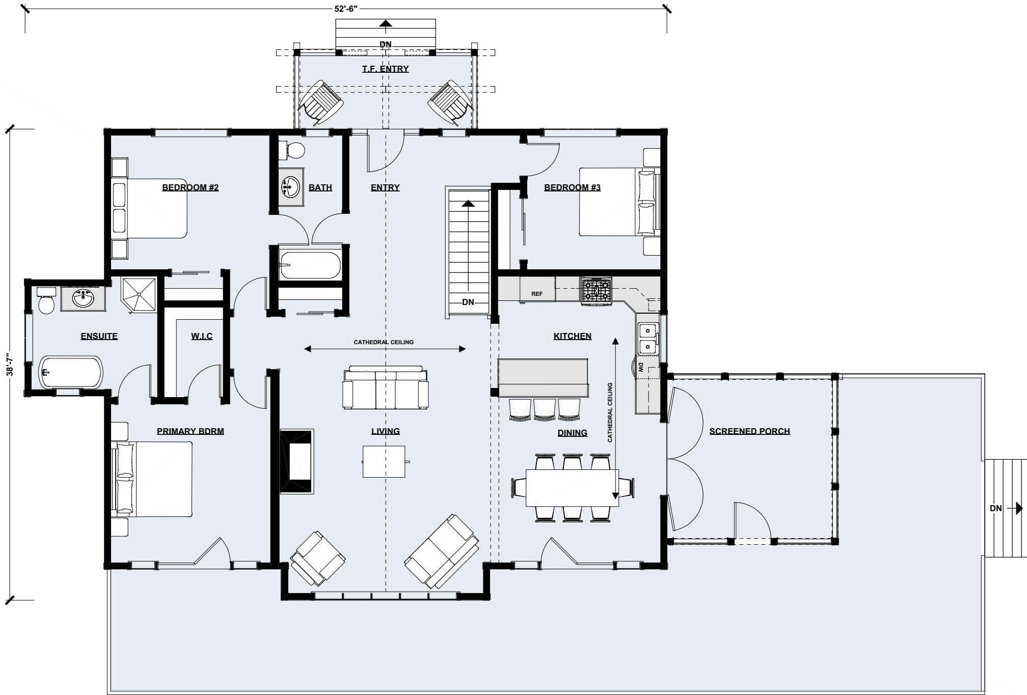
Main Floor Plan | 1,724 sq ft
