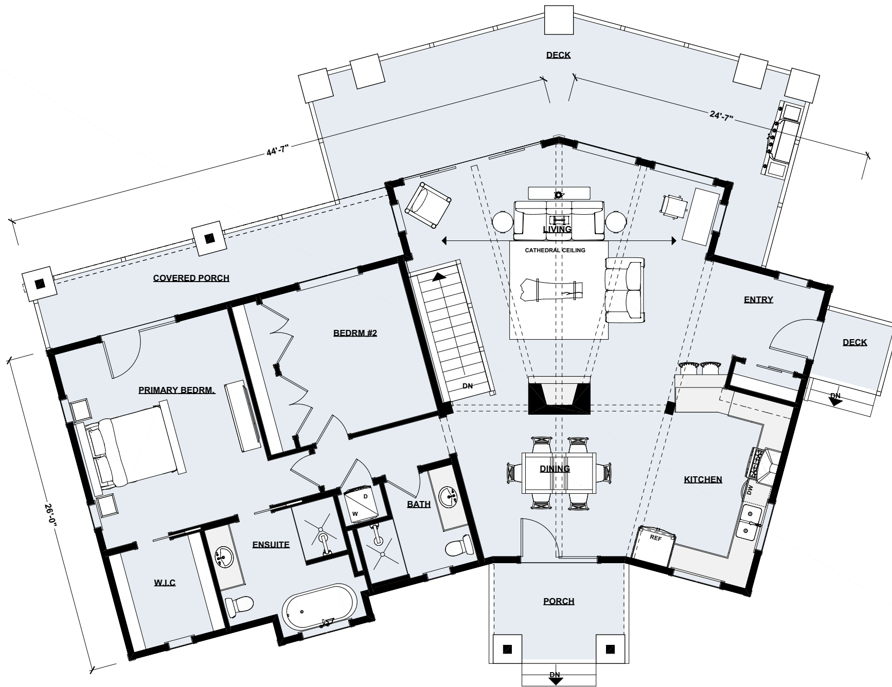
Main Floor Plan | 1,680 sq ft
