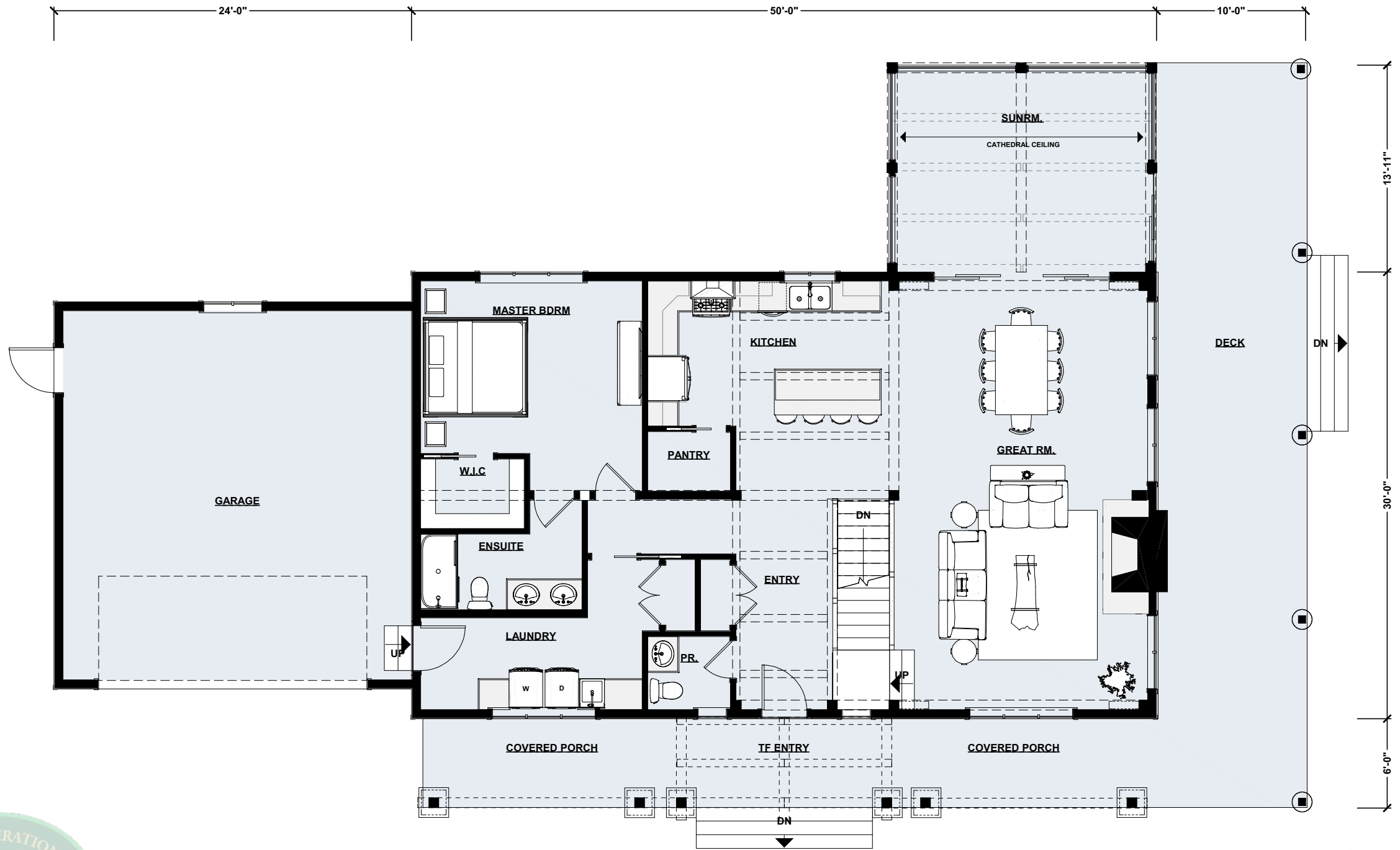
Main Floor Plan | 1678 sq ft
