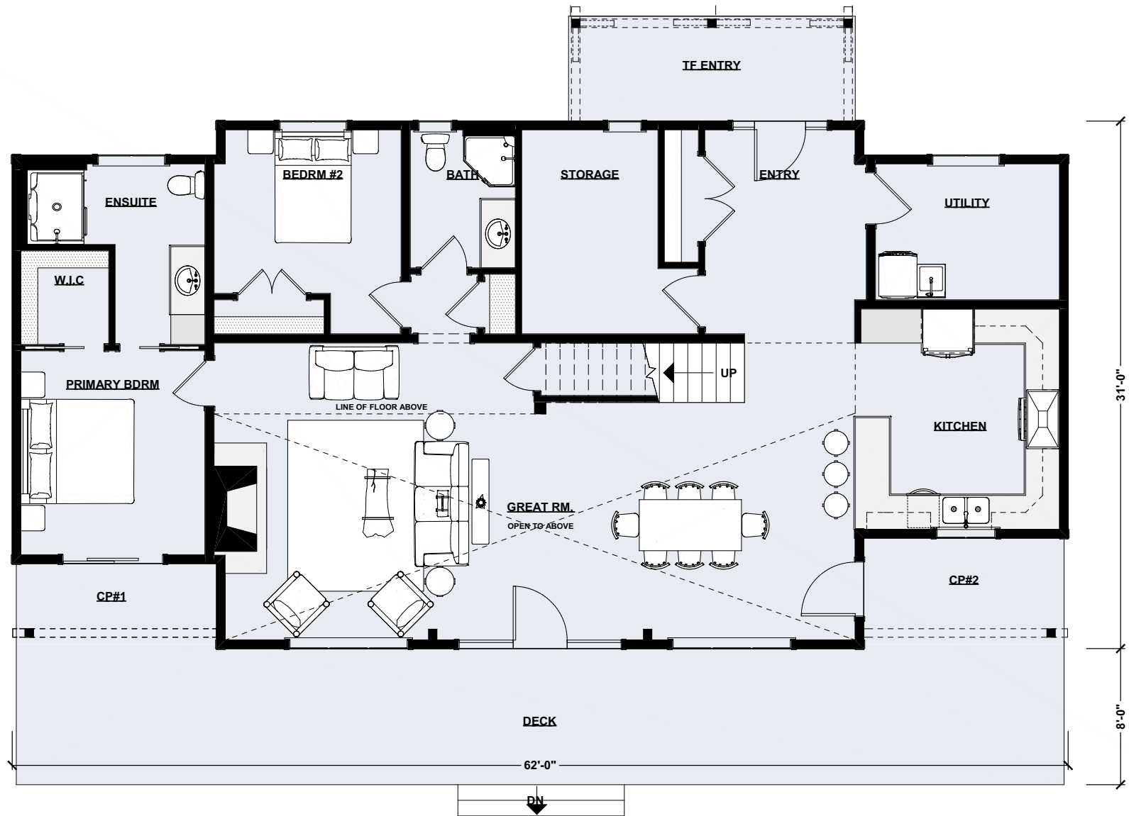
Main Floor Plan | 1,736 sq ft
