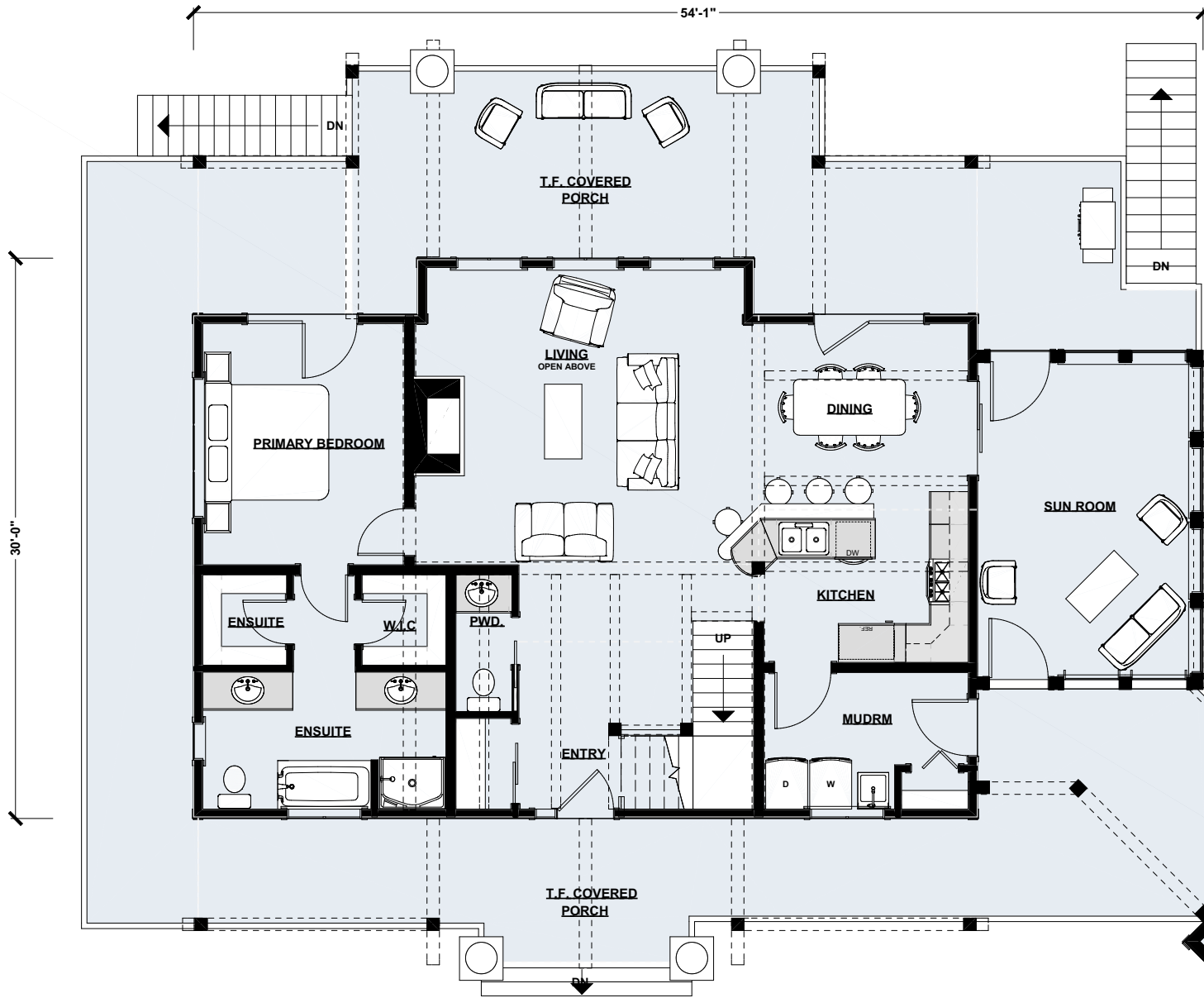
Main Floor Plan | 1,399 sq ft
