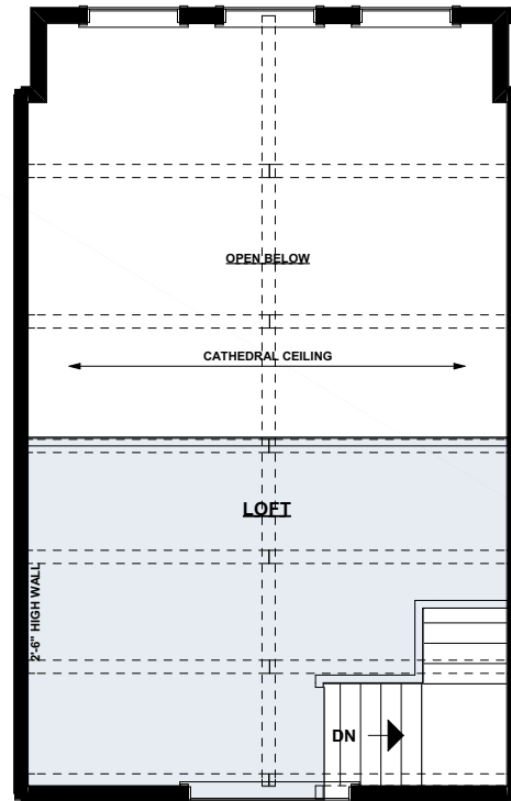
Upper Floor Plan | 211 sq ft
