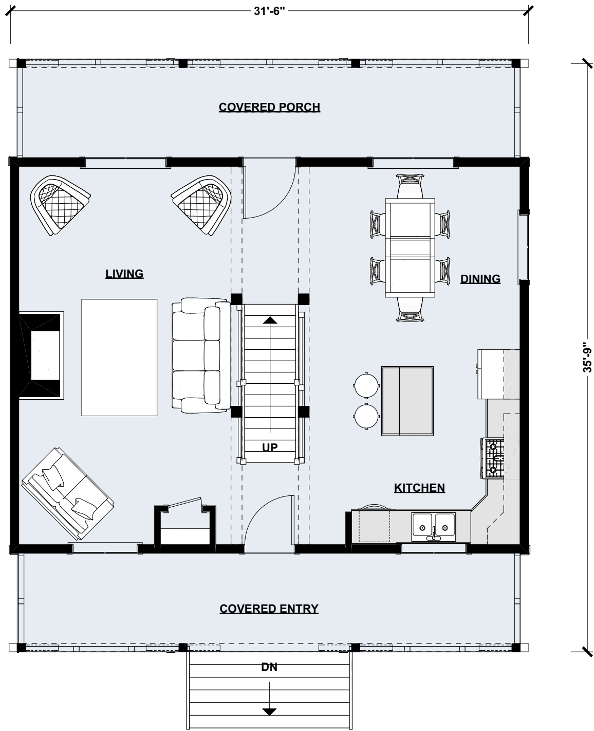
Main Floor Plan | 725 sq ft
