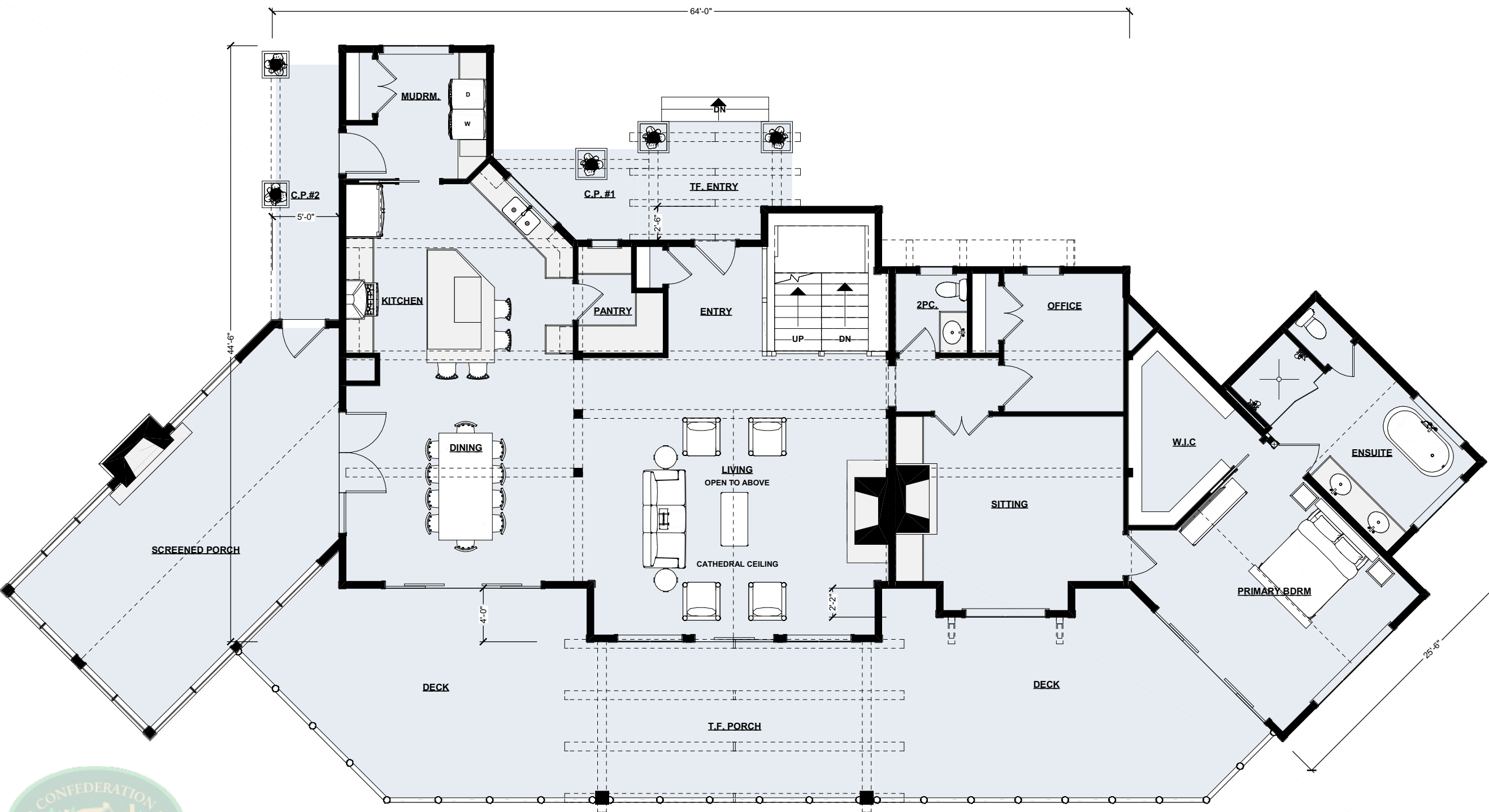
Main Floor Plan | 2264 sq ft
