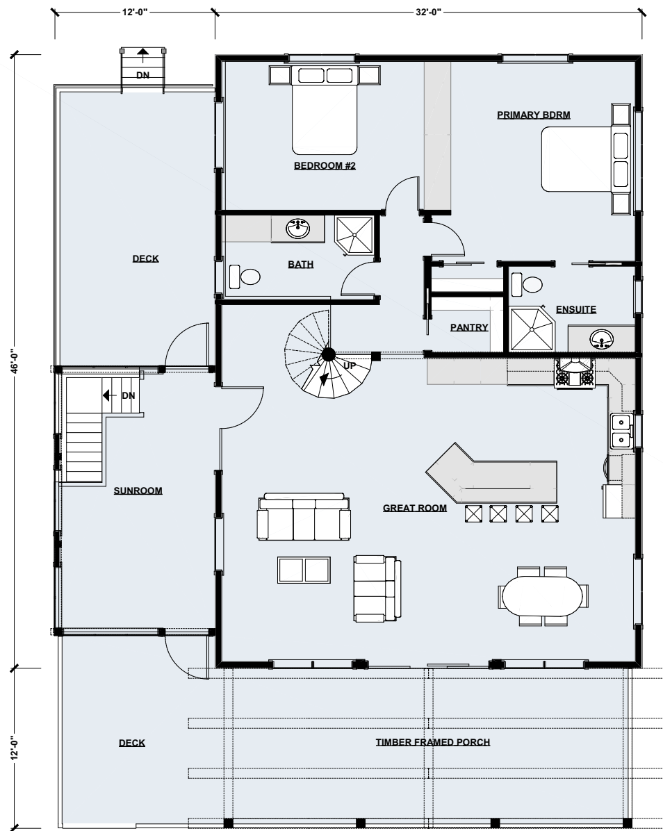
Main Floor Plan | 1,472 sq ft
