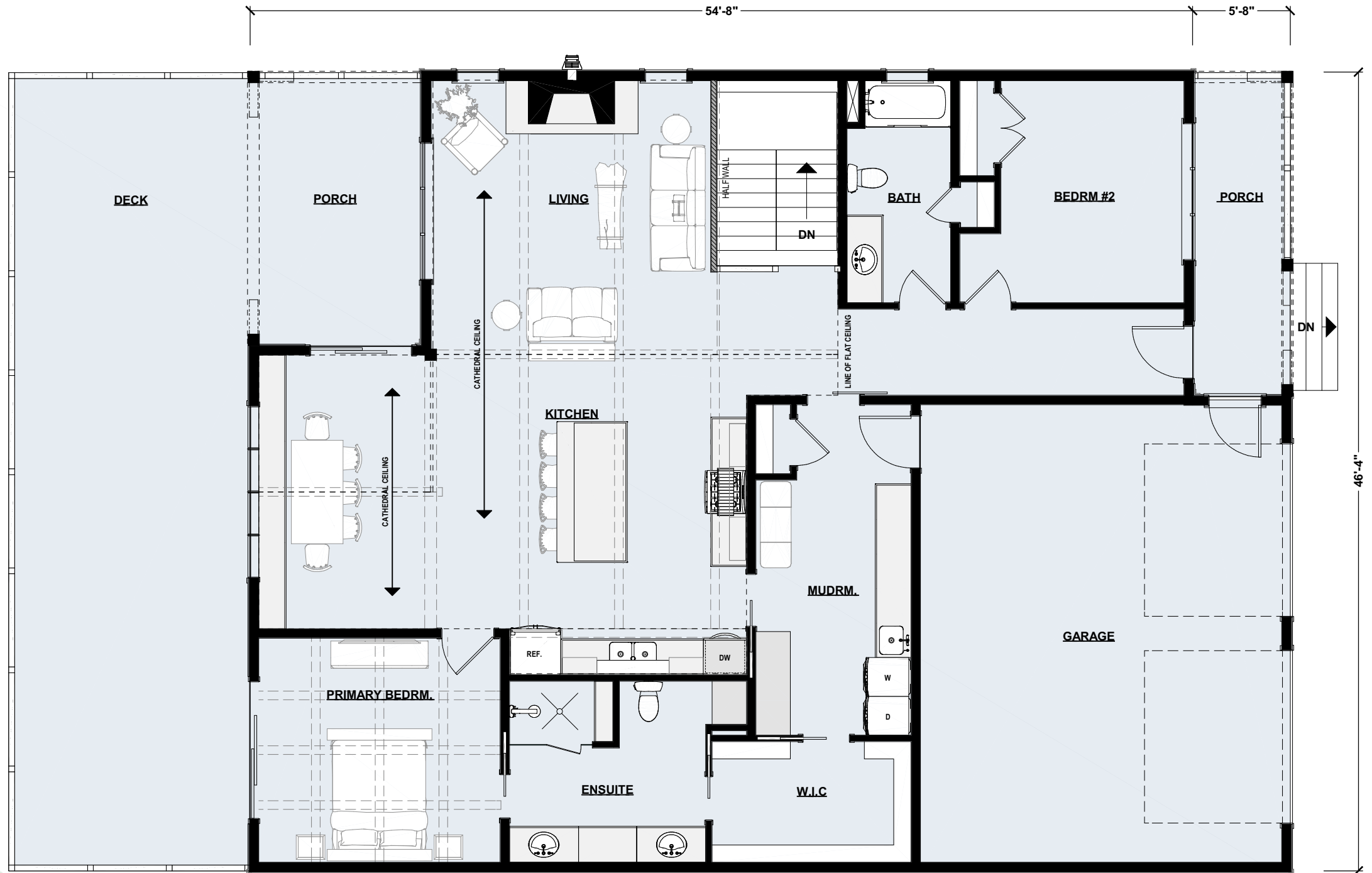
Main Floor Plan | 1863 sq ft
