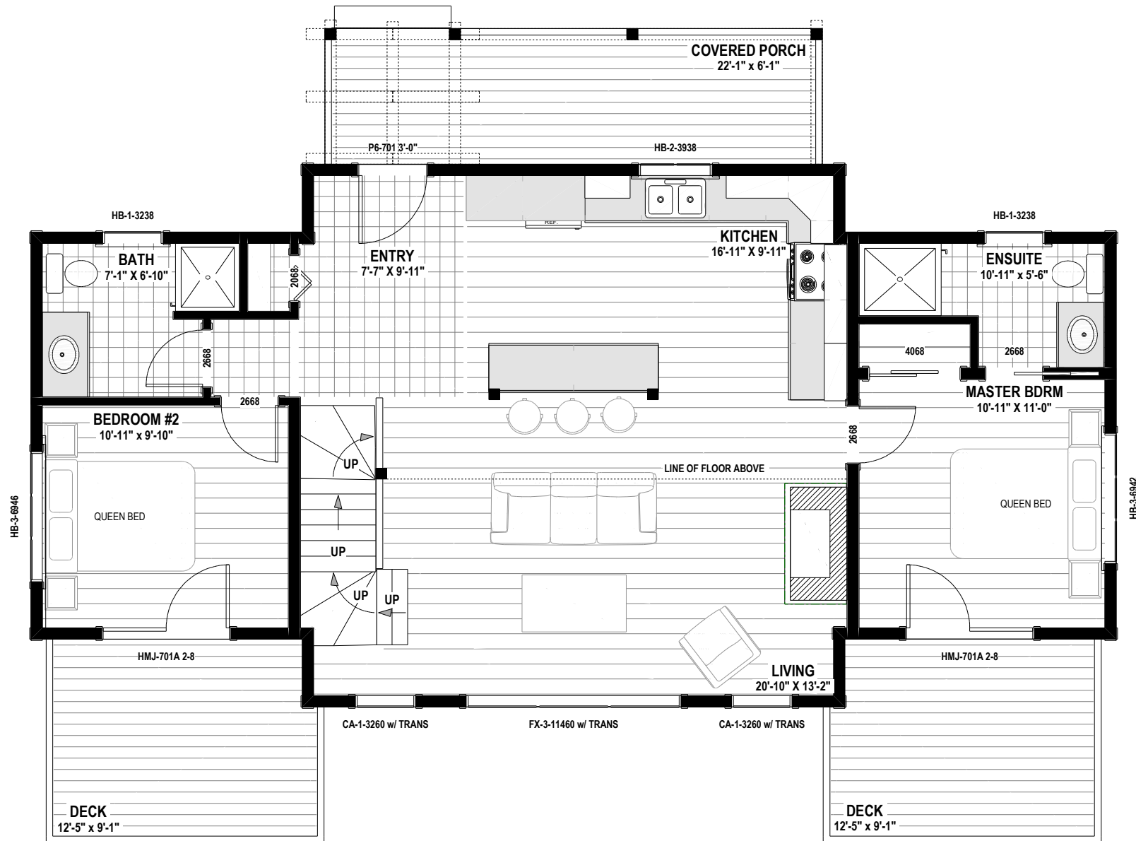
MAIN FLOOR PLAN LIVING AREA = 1008 SQ.FT
