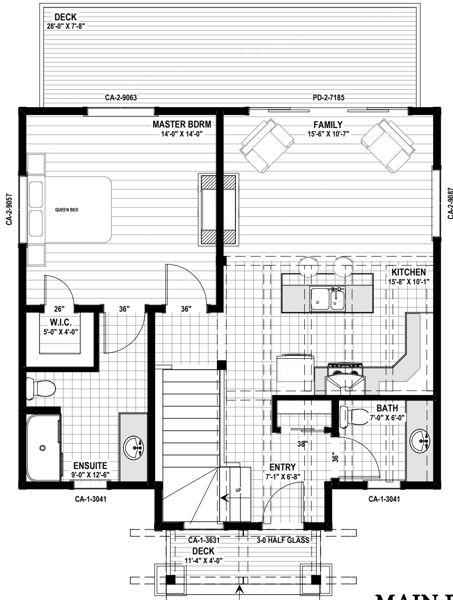
MAIN FLOOR PLAN 907 SQ.FT
