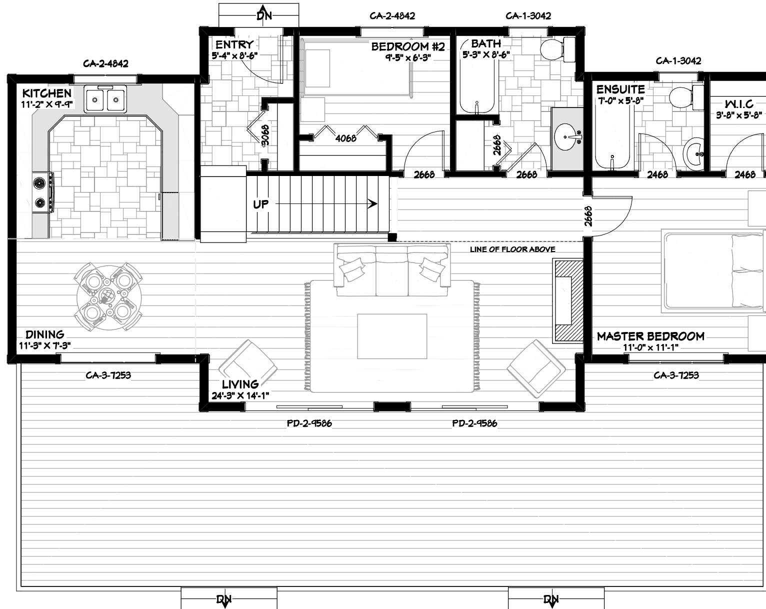
MAIN FLOOR PLAN 1008 SQ.FT
