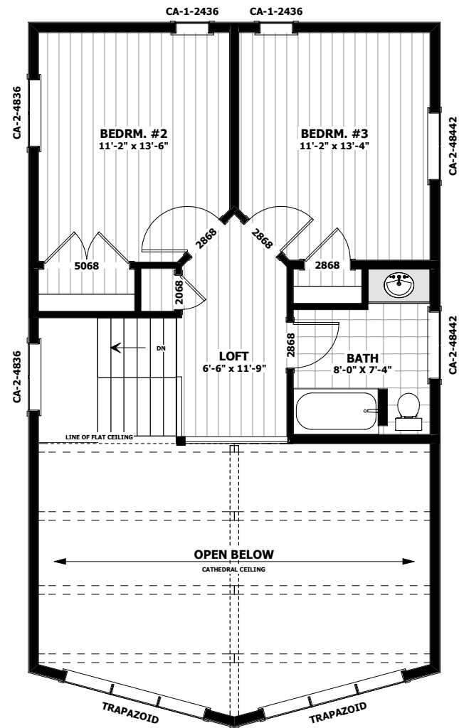
UPPER FLOOR PLAN 526 SQ.FT
