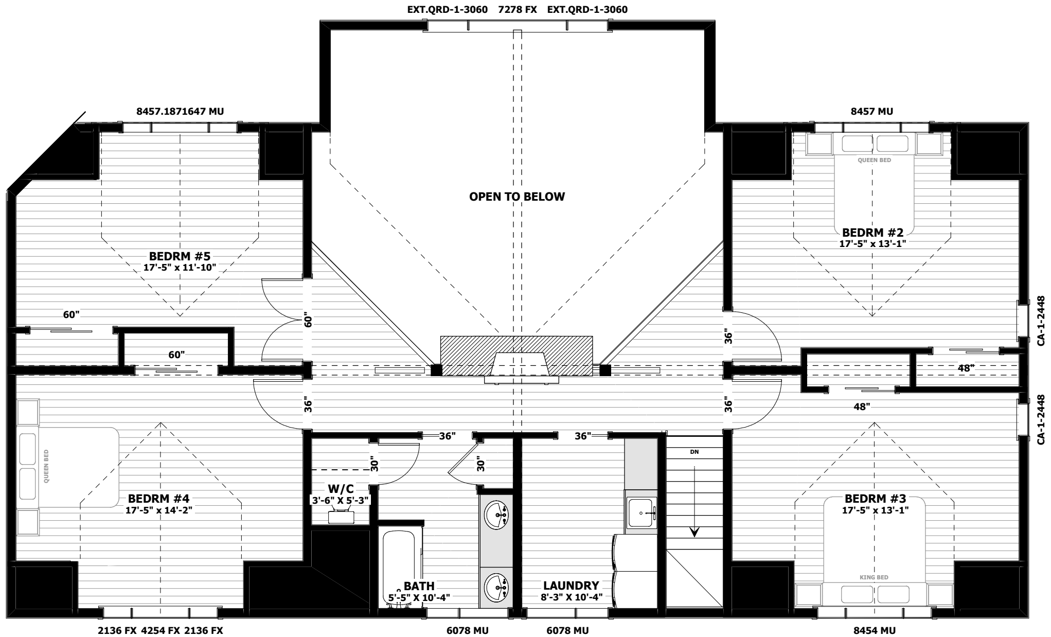
UPPER FLOOR PLAN 1500 SQ.FT
