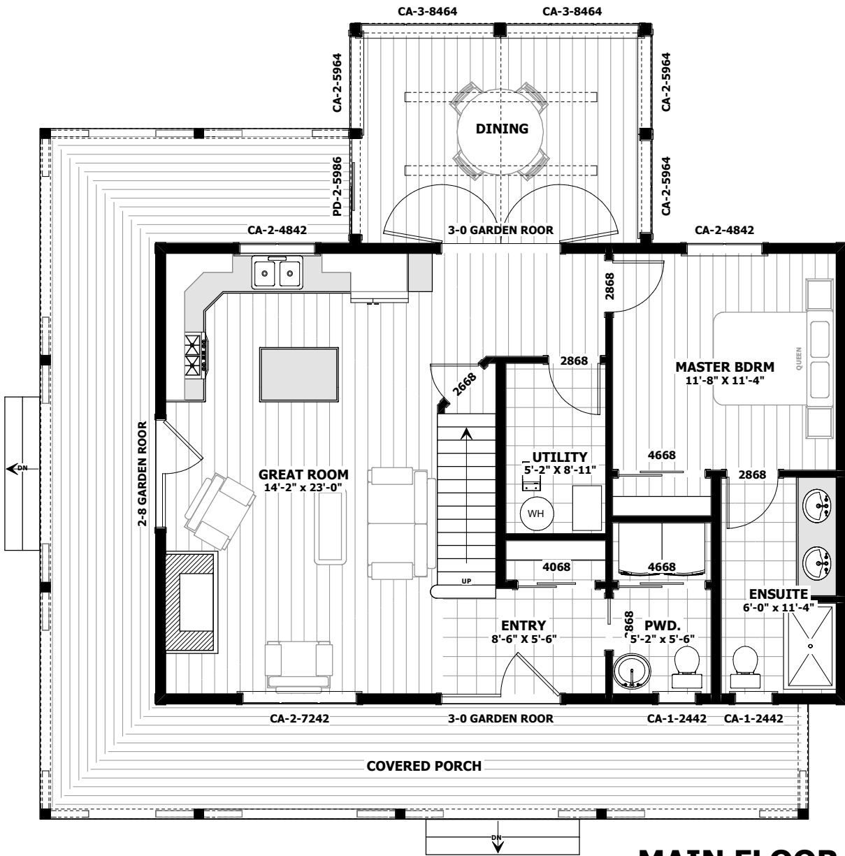
MAIN FLOOR PLAN 1042 SQ.FT
