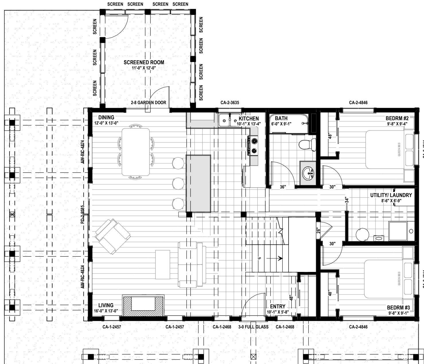
MAIN FLOOR PLAN 1134 SQ.FT
