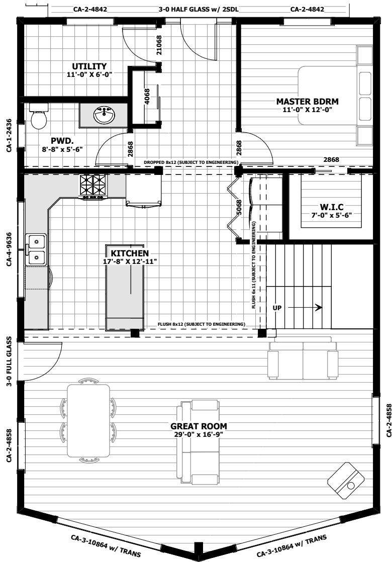
MAIN FLOOR PLAN 1290 SQ.FT
