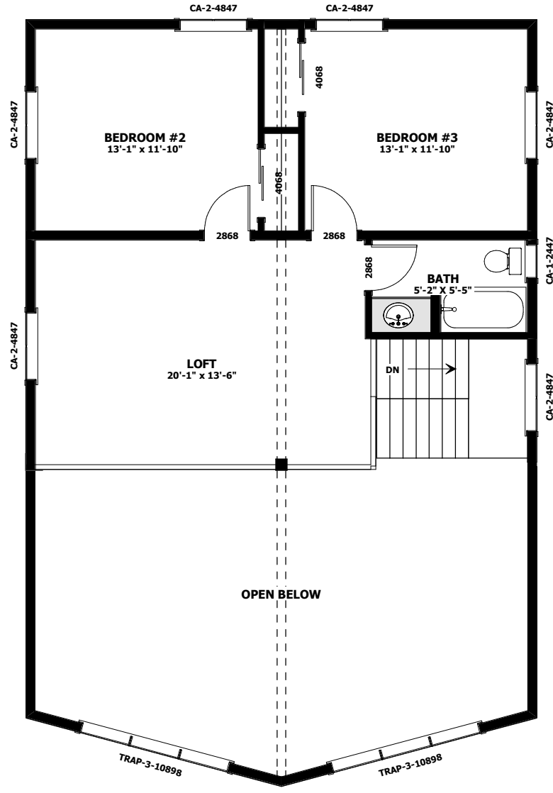
UPPER FLOOR PLAN 721 SQ.FT
