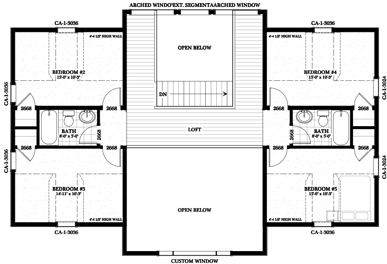
UPPER FLOOR PLAN 1106 SQ.FT
