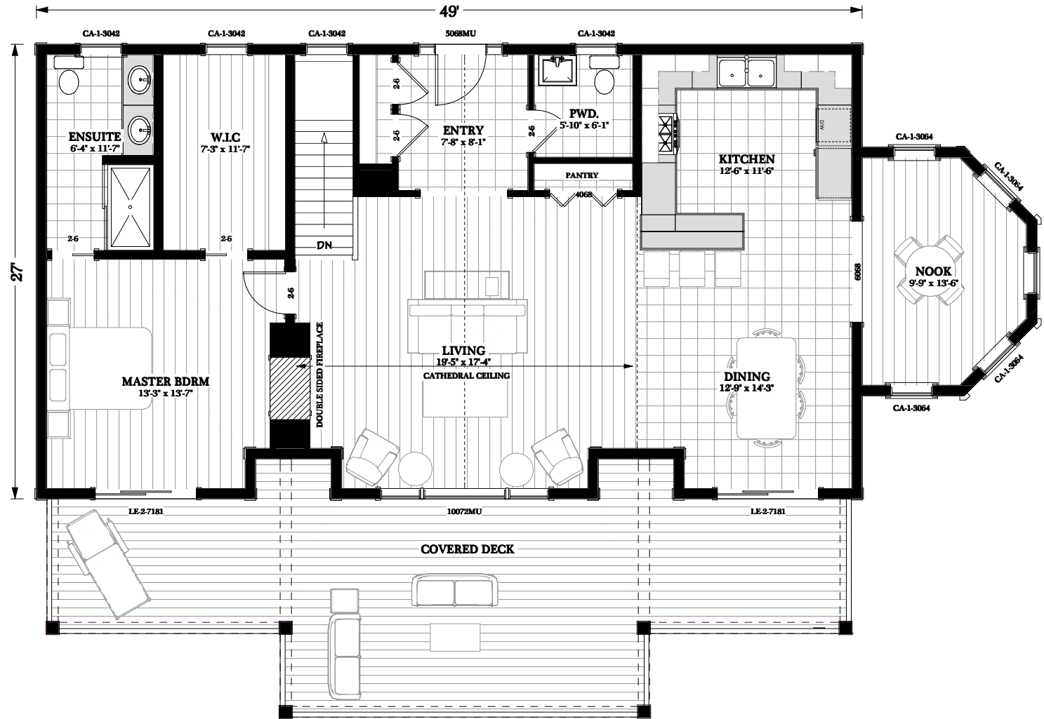
MAIN FLOOR PLAN 1437 SQ.FT
