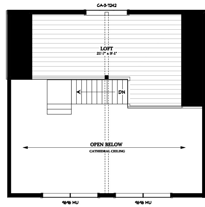
UPPER FLOOR PLAN 338 SQ.FT
