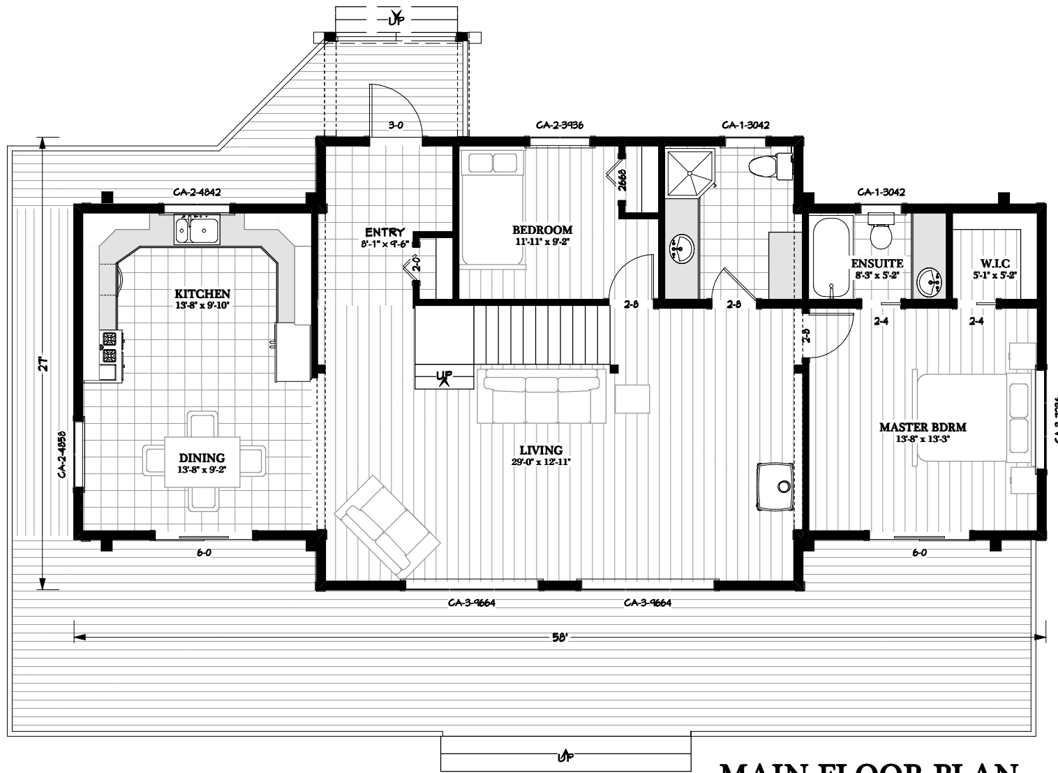
MAIN FLOOR PLAN 1364 SQ.FT
