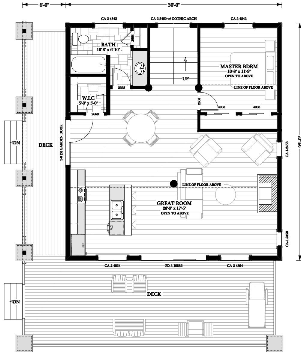
MAIN FLOOR PLAN 990 SQ.FT
