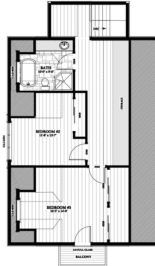
UPPER FLOOR PLAN 826 SQ.FT
