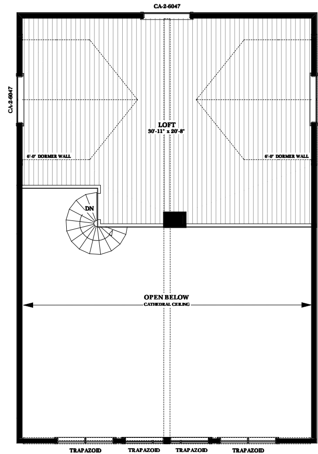
UPPER FLOOR PLAN 698 SQ.FT
