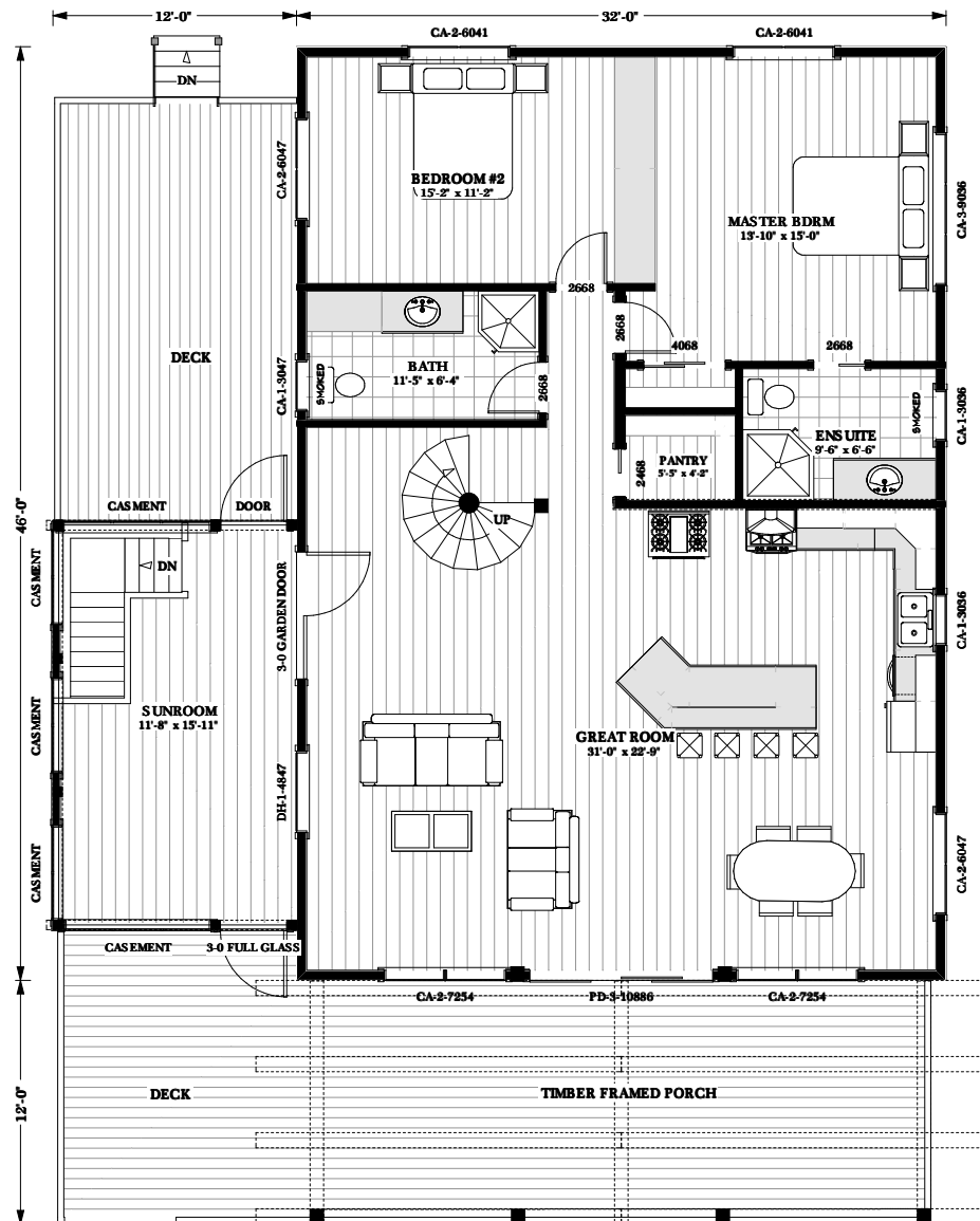
MAIN FLOOR PLAN 1472 SQ.FT
