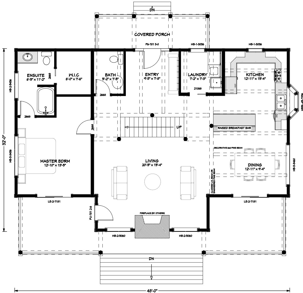
MAIN FLOOR PLAN 1368 SQ.FT
