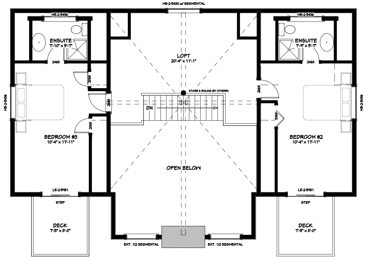
UPPER FLOOR PLAN 1002 SQ.FT
