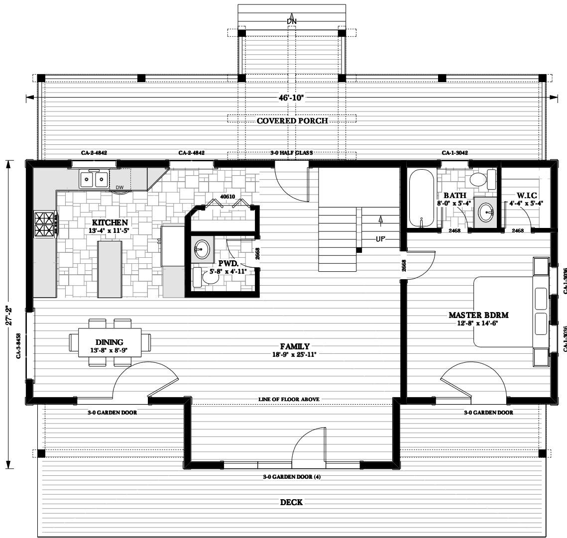
MAIN FLOOR PLAN 1115 SQ.FT
